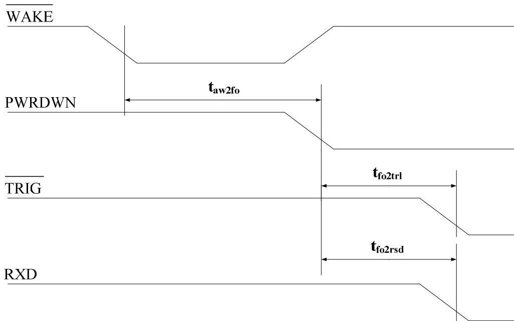
Figure 4-8 Wake-up timing
