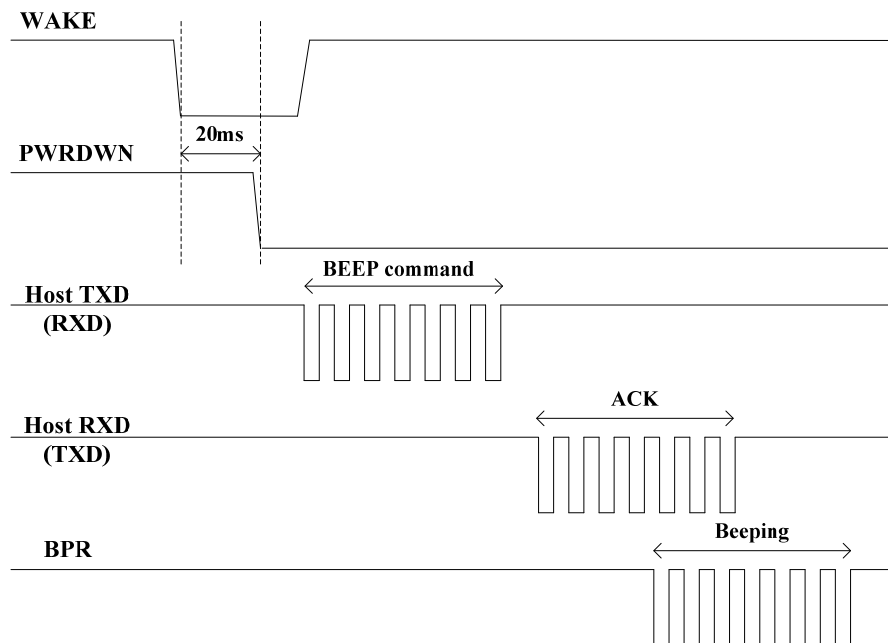
Figure 5-1 Wake and beep timing
