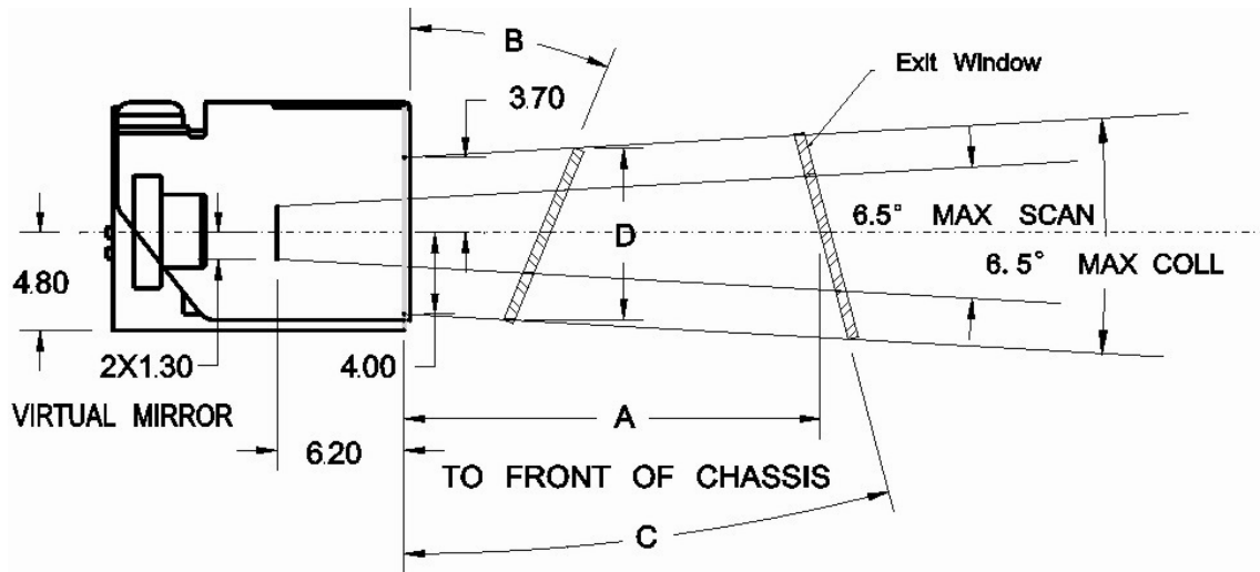
Figure 3-2 Exit window tilt angle
