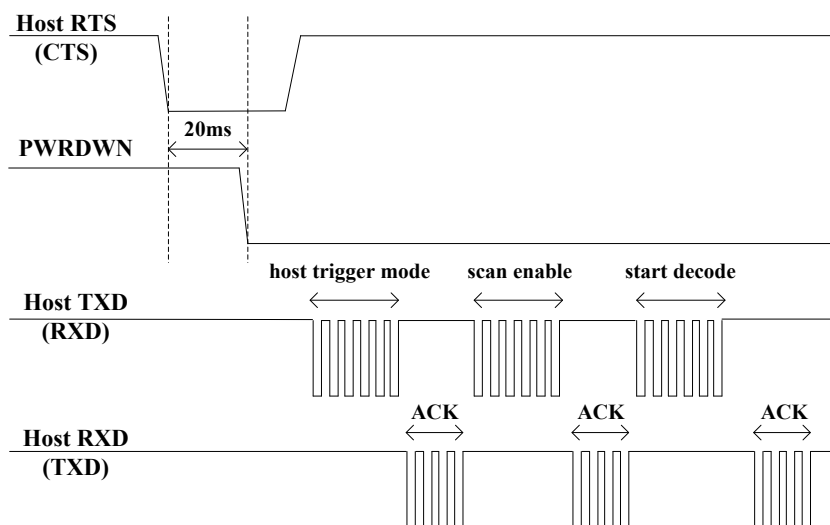
Figure 5-3 STRAT_DECODE timing
