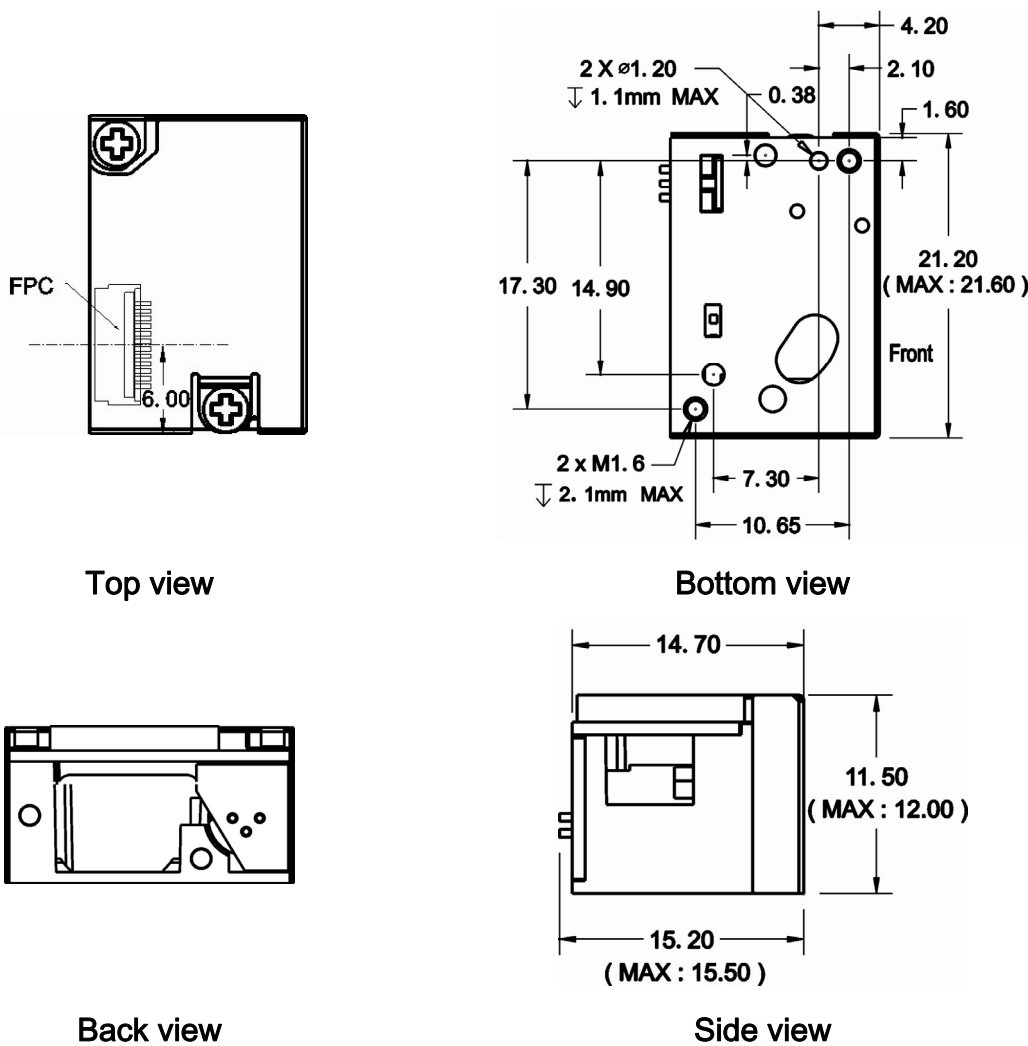
Figure 3-1 Mounting diagram
