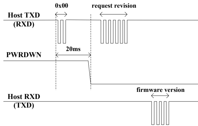
Figure 5-2 REQUEST_REVISION timing
