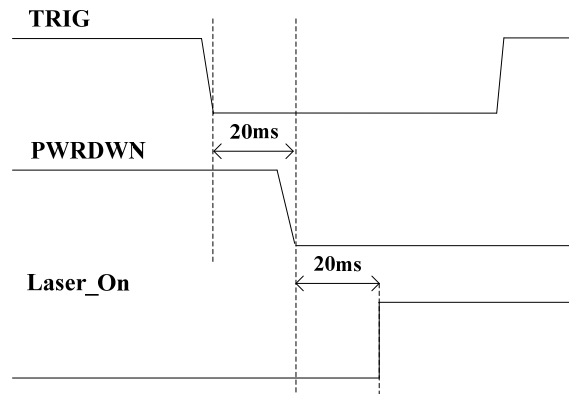
Figure 5-4 TRIG pulled down to start decode timing
