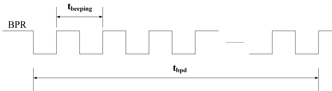
Figure 4-5 Beeper timing
