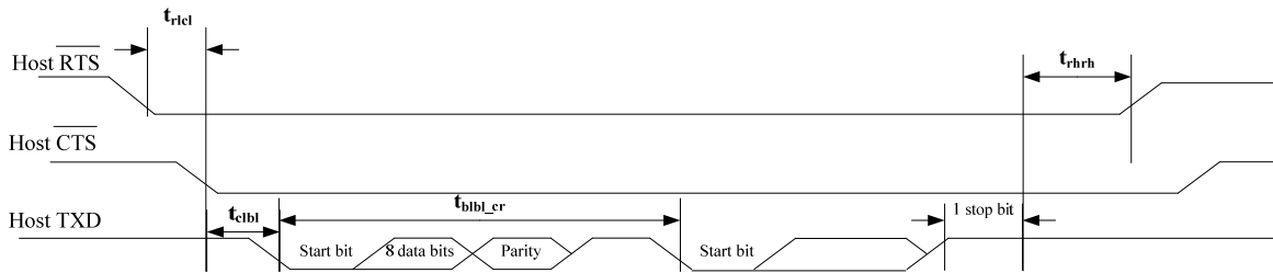
Figure 4-2 Serial I/O timing
